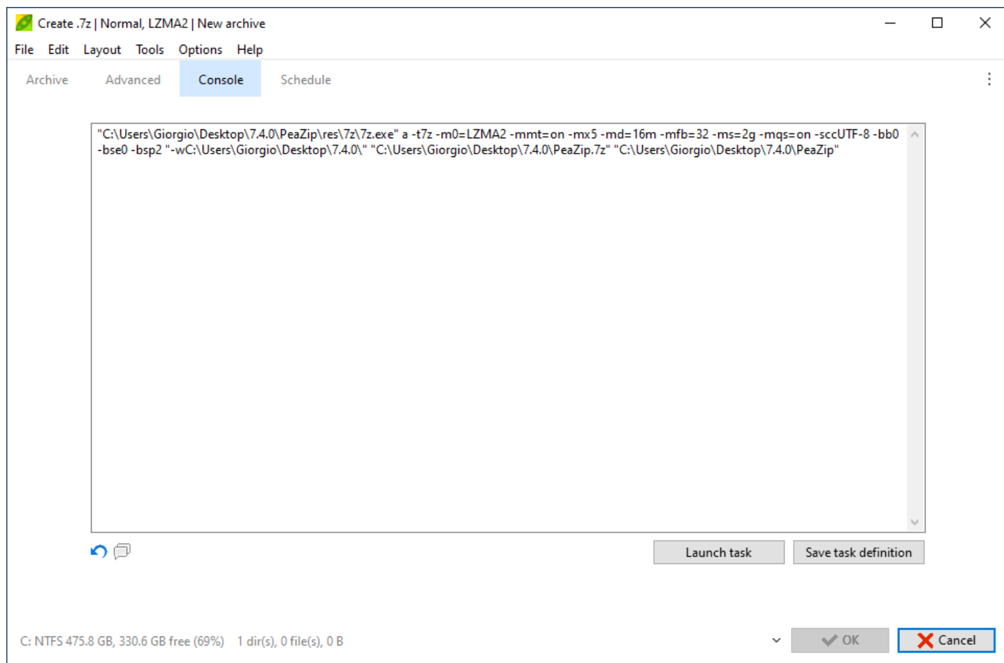
Image 17: Console tab: the command line corresponding to the task generated in the GUI
