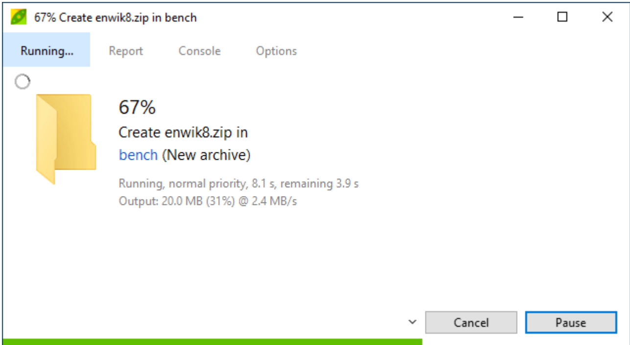
Image 19: PeaLauncher instance
