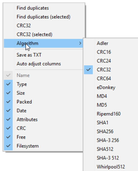
Image 10b: Headers' context menu
