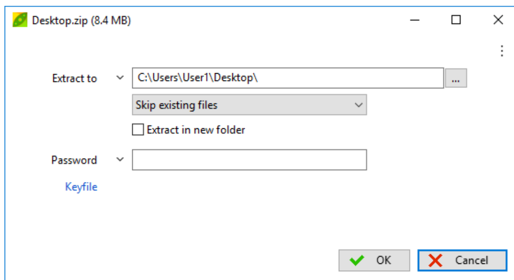
Image 21: PeaExtractor
