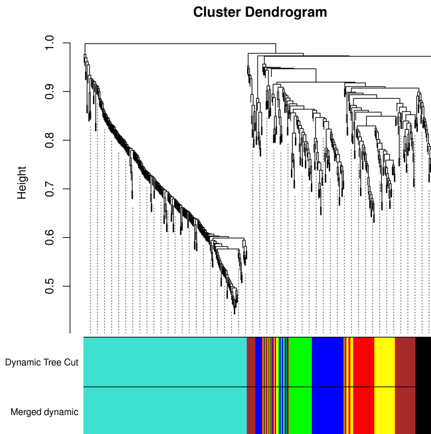
Figure 1: Cluster dendrogram
